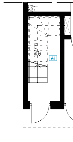
PARTER
